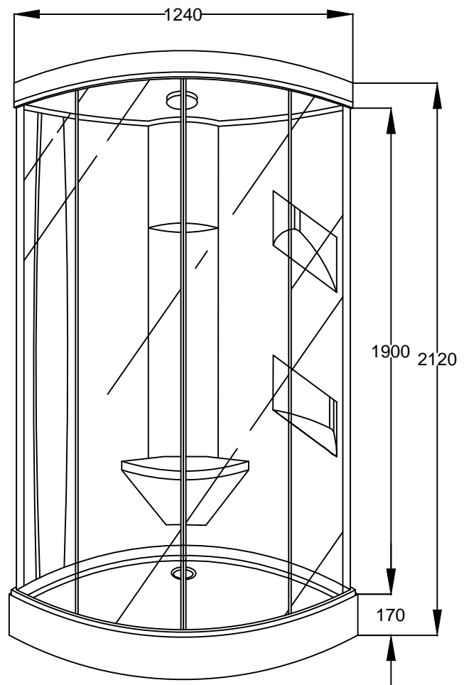
BARI 1000x1000x2120 mm
